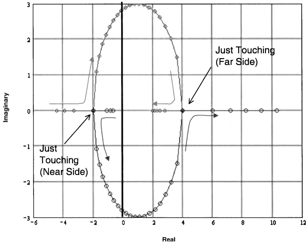
Fig. 1 Representative locus of admissible eigenvalues.
